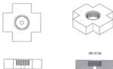
8" SQUARE X 1 1/2" ROTOR PART #8827T
